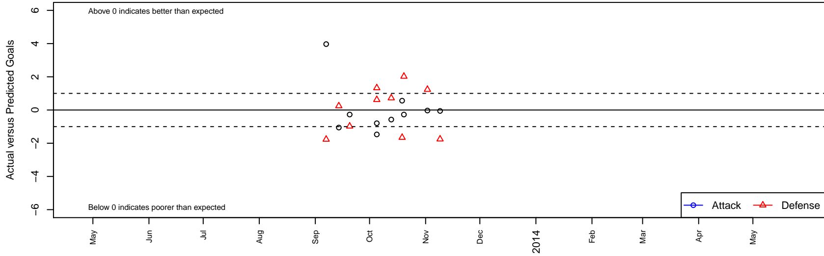
Ajax United 03 Green G02 Dots are actual minus expected GF (blue circles) and GA (red triangles). Blue line is smoothed change in attack strength. Red is smoothed change in defense strength.
